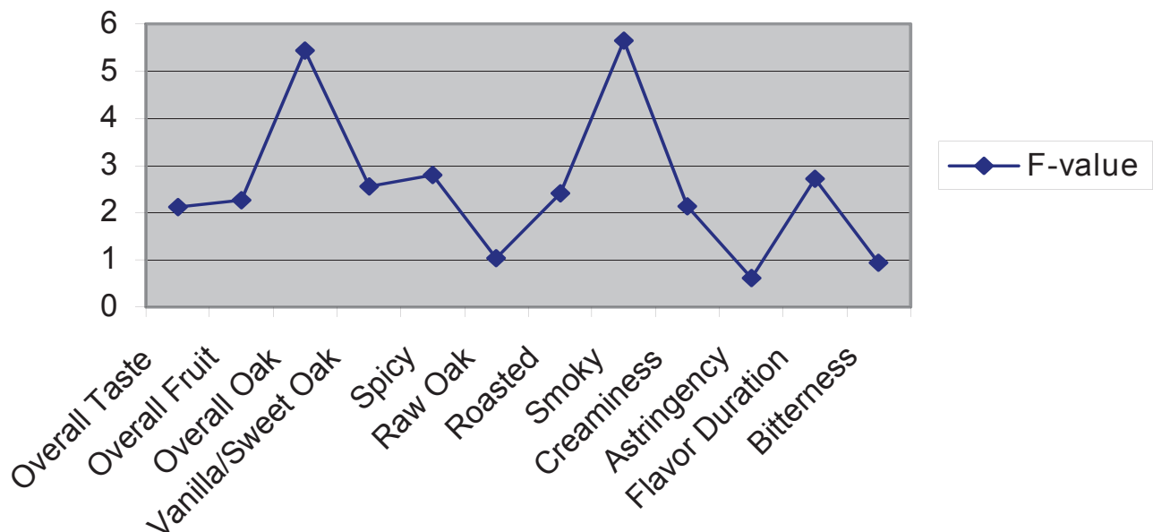
Figure 1: Red Wine F-values based on 12 Red wine attributes, n= 42 judges, \alpha = 0.05 .
